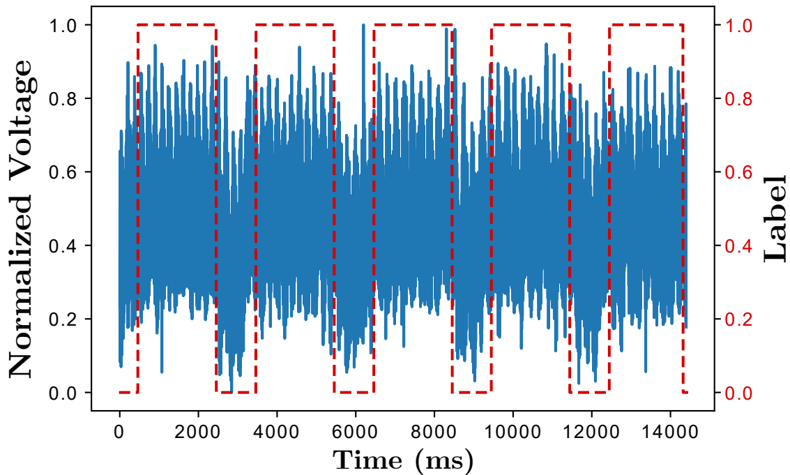
Normalized Data for SSH Login Attempts in Time-Domain (DC)
