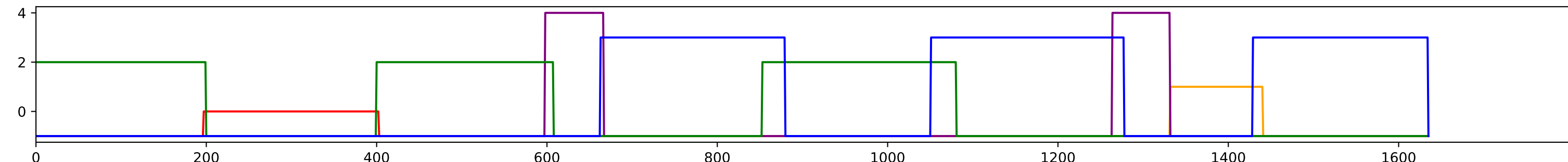
Activations
