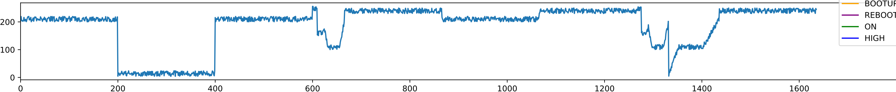
Initial Trace
