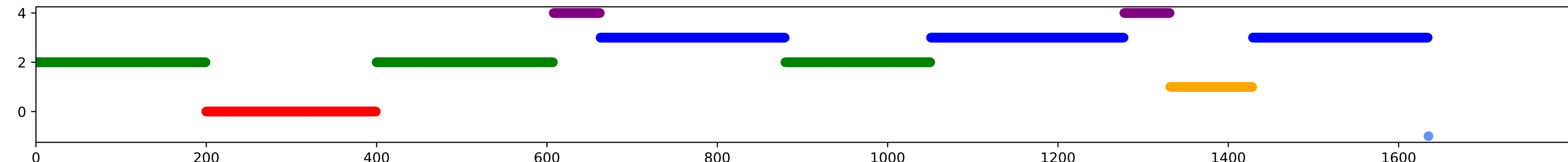
Final labels
